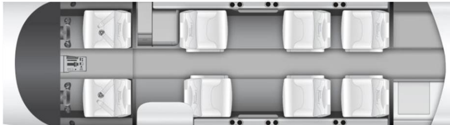
8 Seat Configuration: 2 Crew Seats and 6 Pedestal Seats
